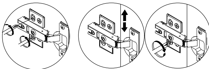
Cabinet door up and down fine adjustment
